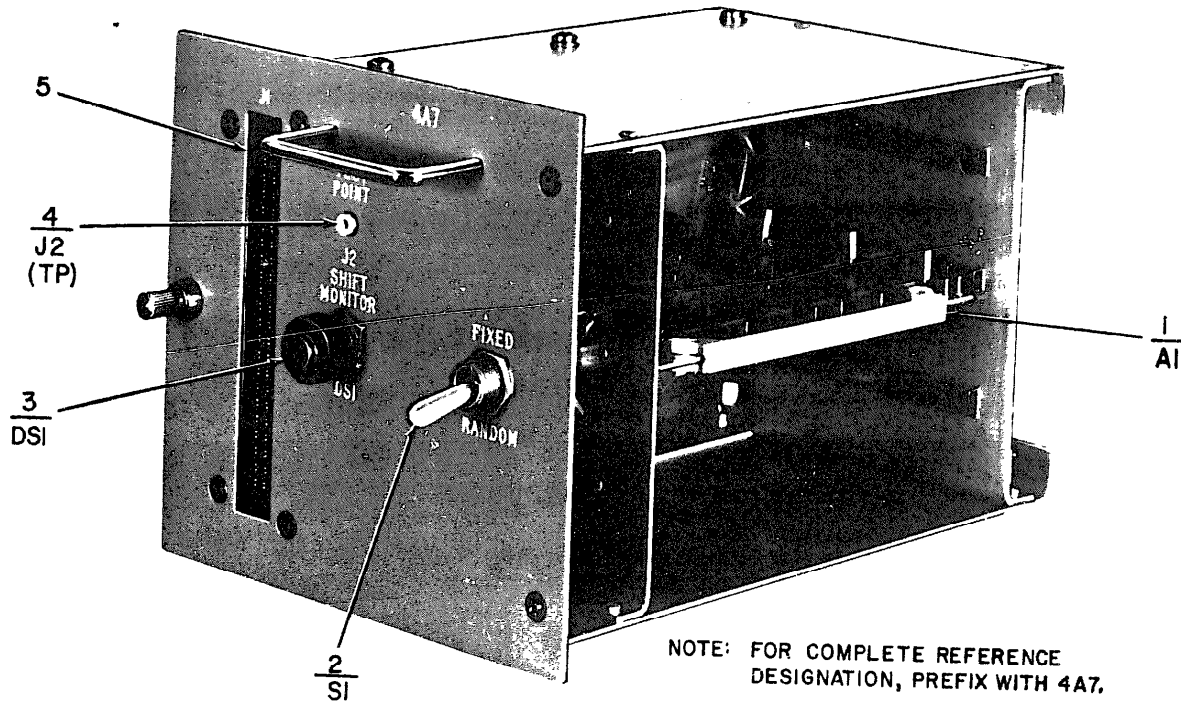
Figure 65 Test Adapter MX-8620/APS-94D 4A7
