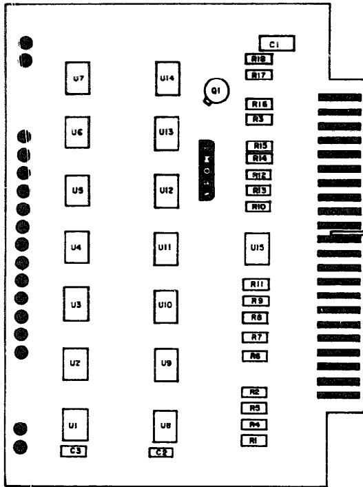
Figure 62 Test signal generator 4A6A1
