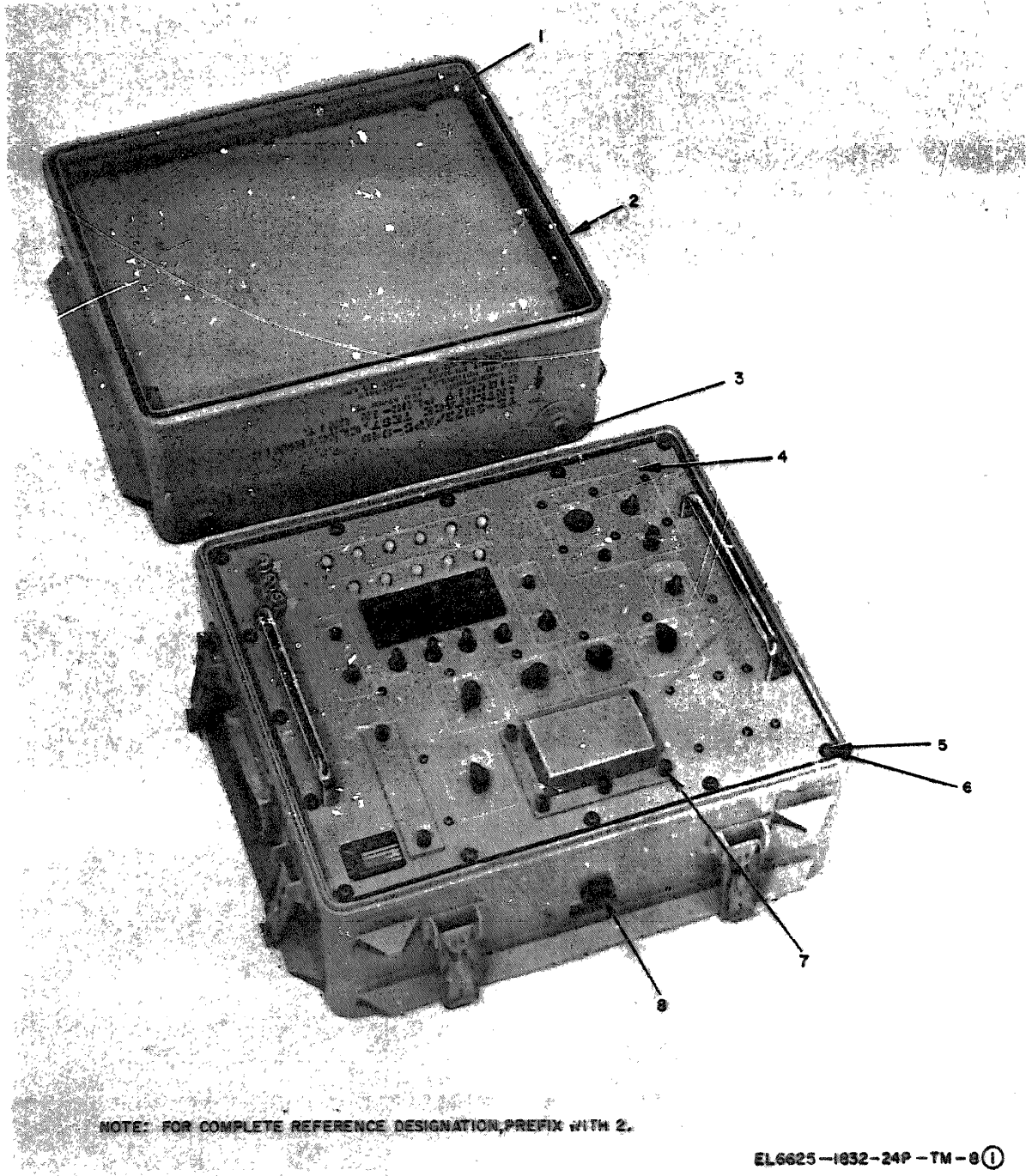
Figure 8 (1) Interface Test Electronic Circuit Plug-in Unit TS-2972/APS-94D (sheet 1 of 2)
