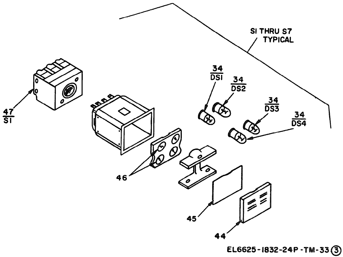
Figure 33 ③ Panel, test, electrical (sheet 3 of 3)
