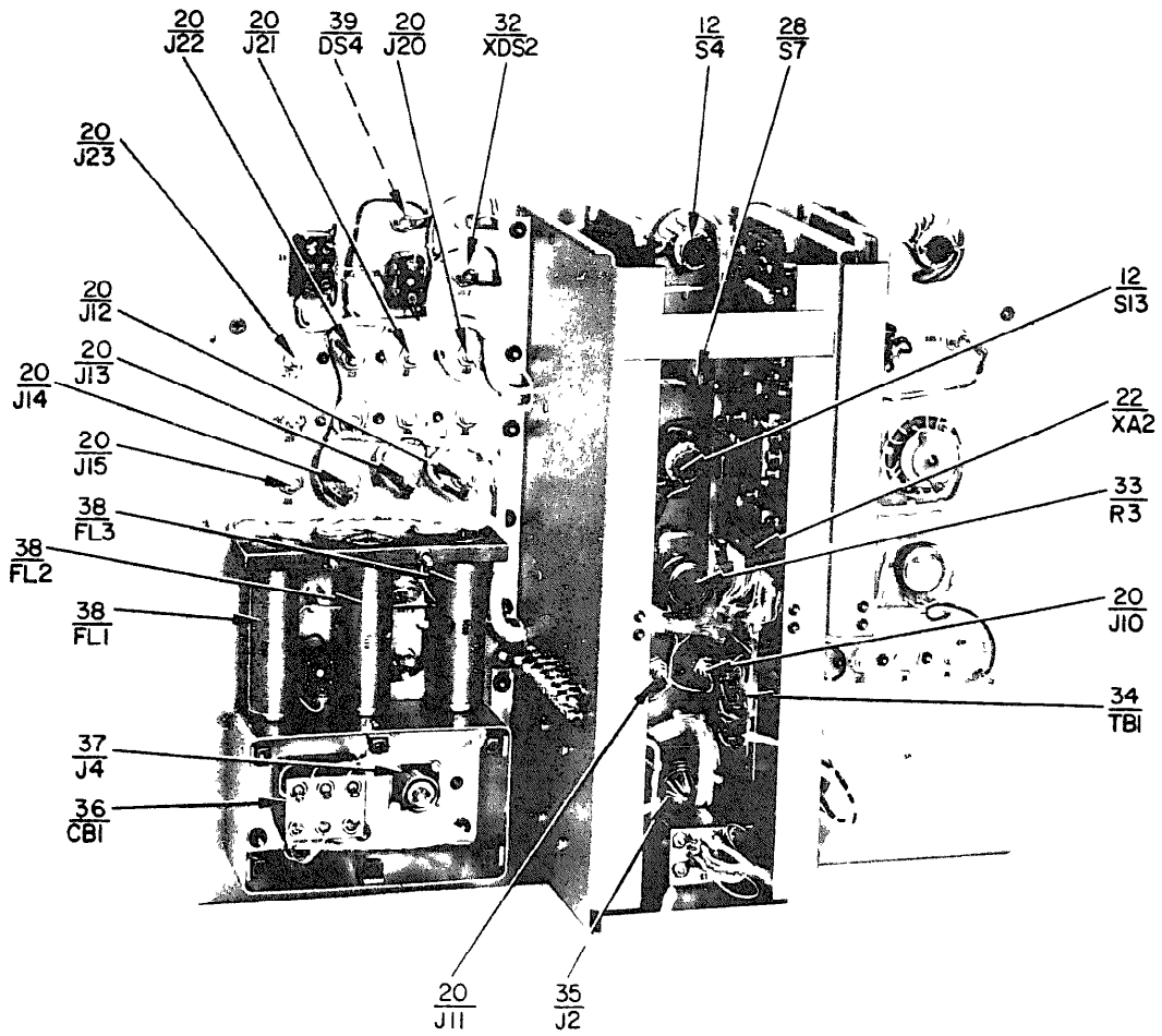
Figure 3. Panel, test, electrical (sheet 3 of 3)
