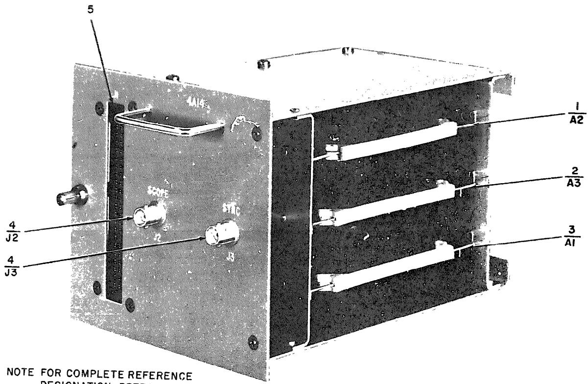
Figure 86 Test Adapter MX-8627/APS-94D 4A14
